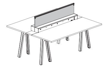
FRONTAL PANEL MELAMINICO/TESSUTO/VERRO FRONTAL PANEL (FABRIC/WOOD/GLASS) PANNEAU FRONTAL (TISSU/BOIS/VERRE) L. 80/100/120/140/160/180/200 - P. 160
